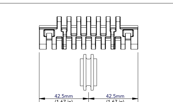
8505/8506 — 85mm — MTW Positrack Tracking Guides
